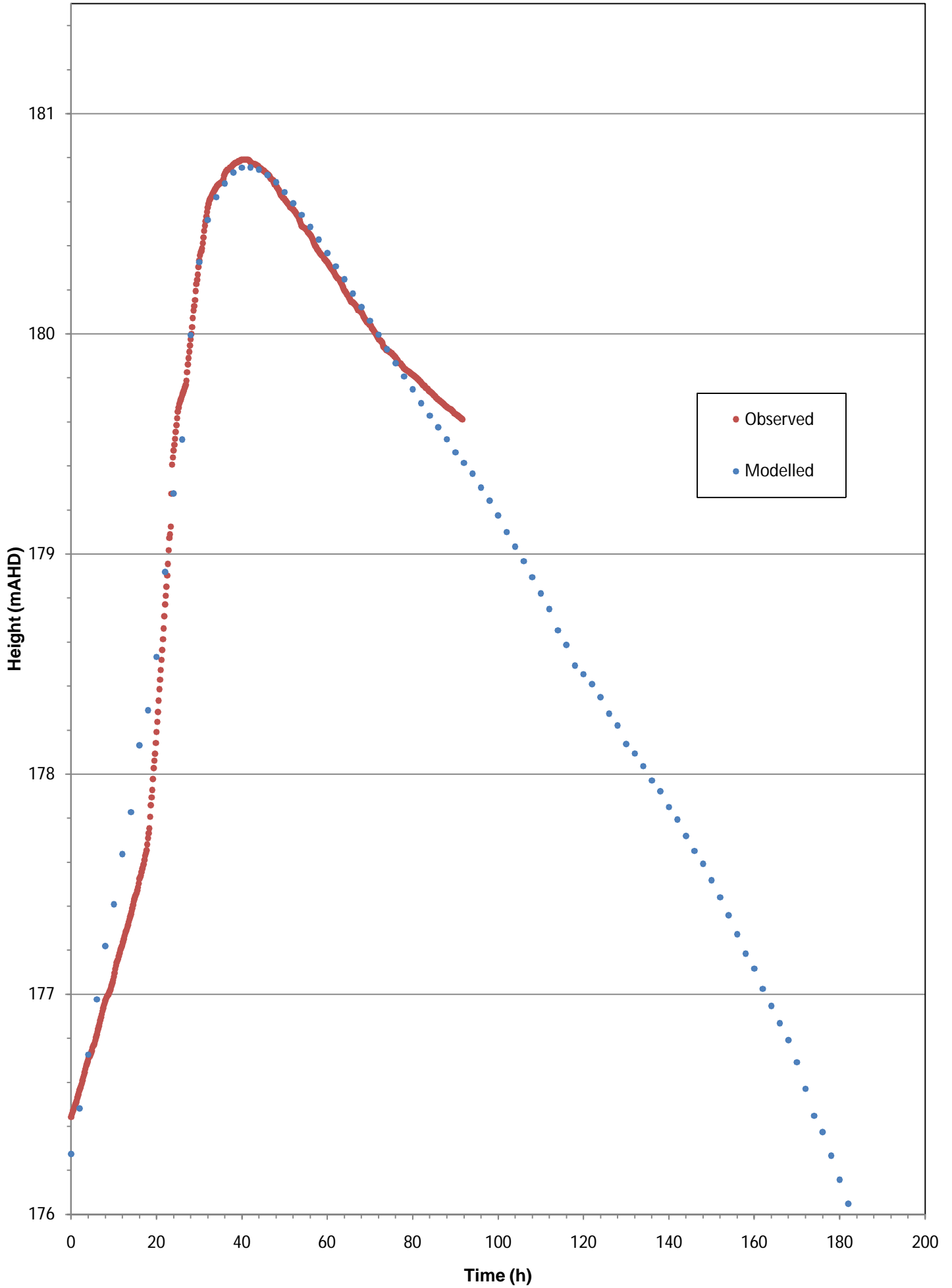
FIGURE 9 Calibration results - 1974 - Hydrograph Comparison
