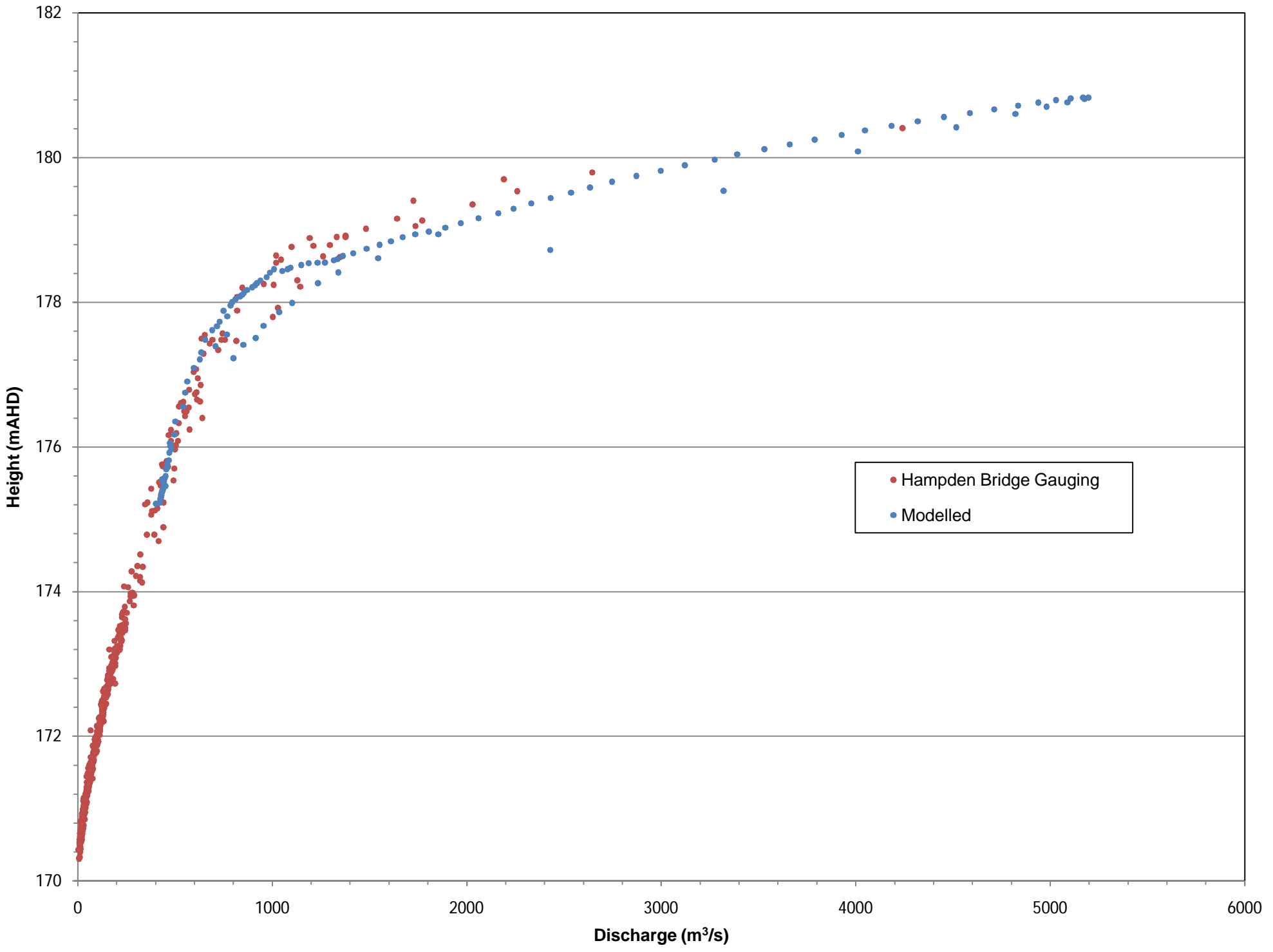
FIGURE 8 Calibration event - 1974 - Stage / Discharge Rating Comparison at Hampden Bridge Gauged vs Modelled
