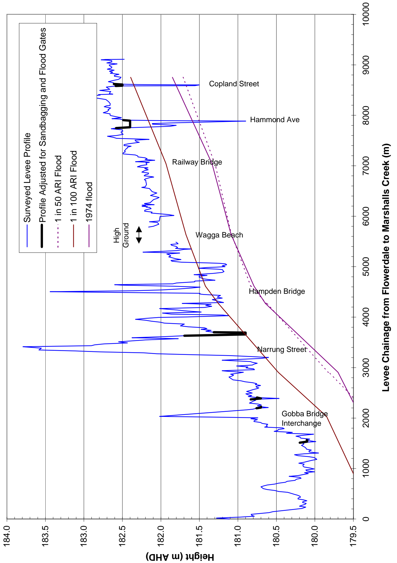
FIGURE 37 MAIN TOWN LEVEL PROFILE DESIGN FLOOD PROFILES
