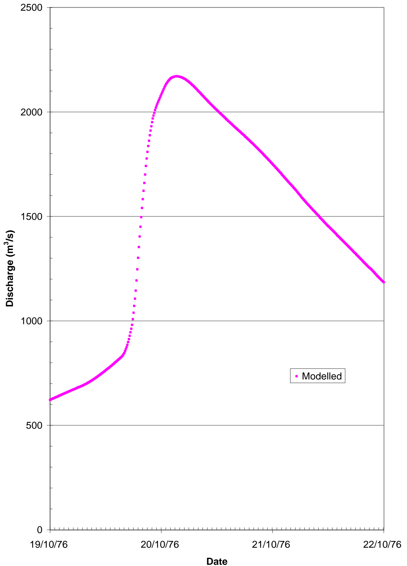
FIGURE 21 DISCHARGE HYDROGRAPH HAMPDEN BRIDGE OCTOBER 1976
