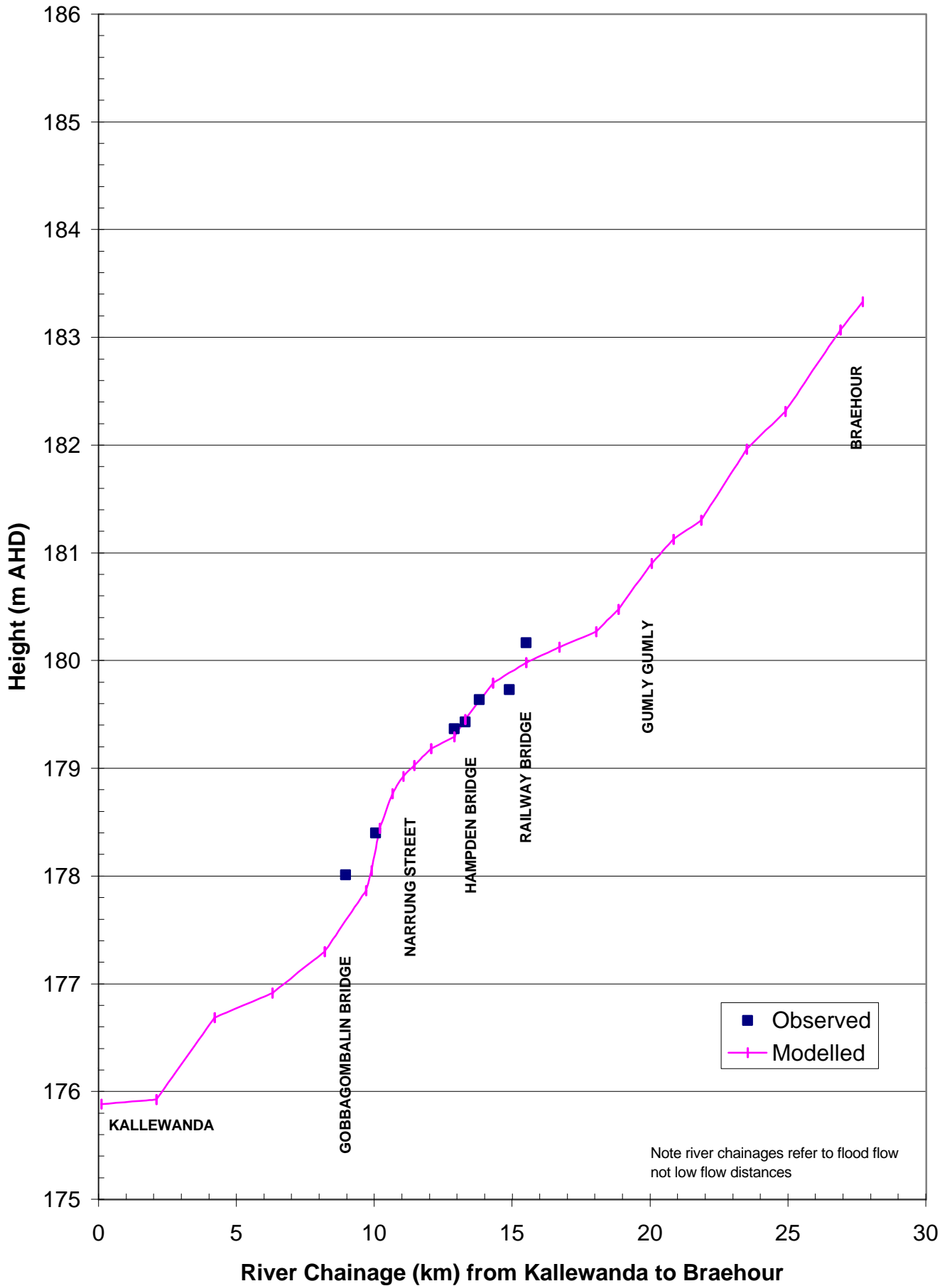
FIGURE 22 PEAK HEIGHT PROFILE OCTOBER 1976
