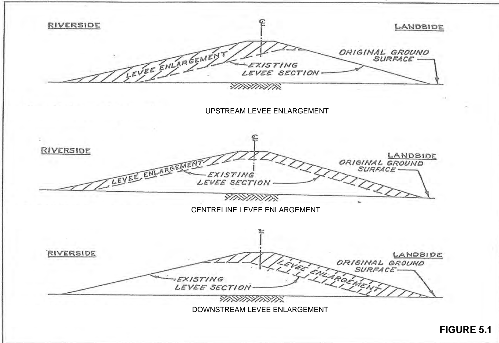
LEVEE UPGRADE ALIGNMENT OPTIONS
