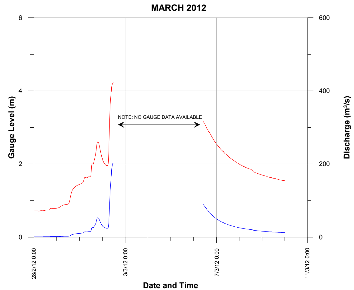
Figure 1.6 STAGE AND DISCHARGE HYDROGRAPHS AT OLD BORAMBOLA GAUGE (GS 410047)
