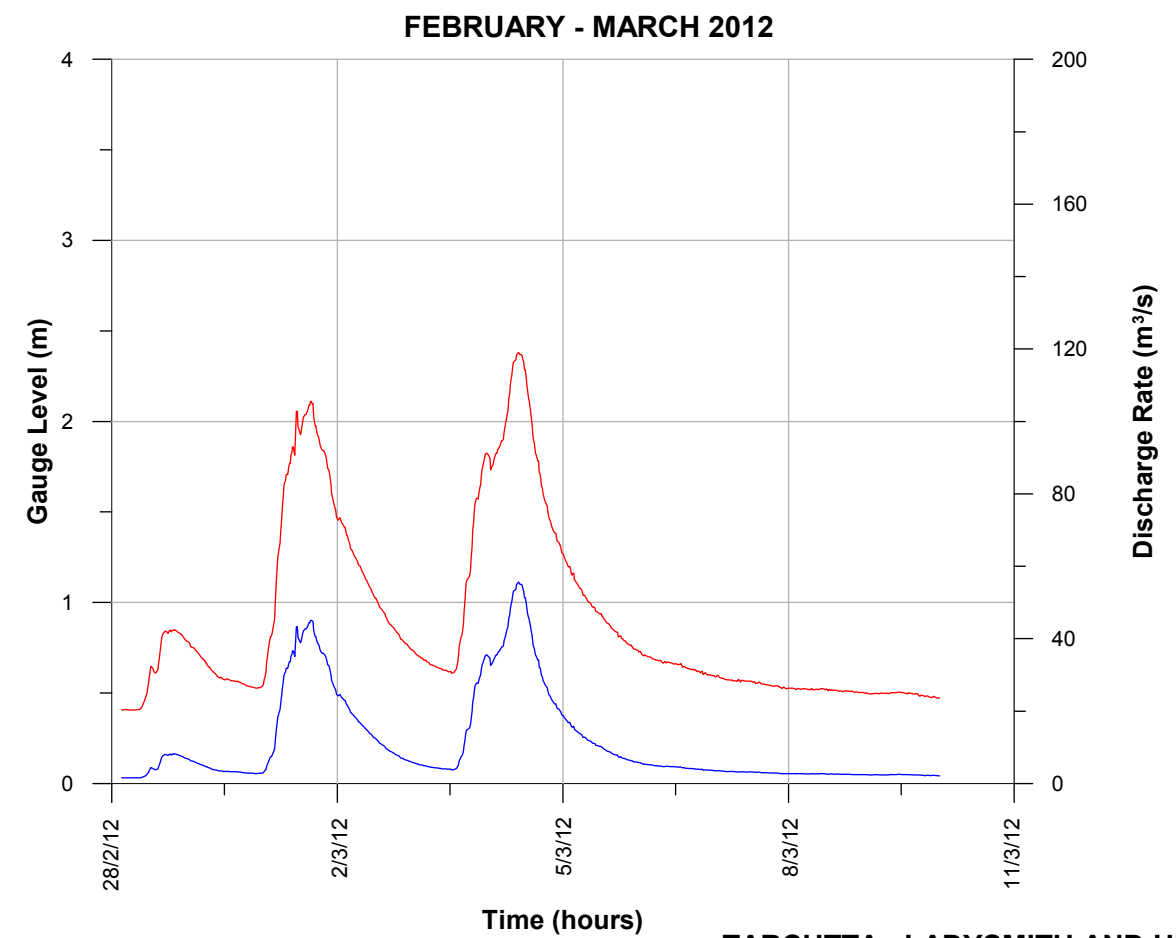
Figure 1.4 STAGE AND DISCHARGE HYDROGRAPHS AT WESTBROOK GAUGE (GS 410058)
