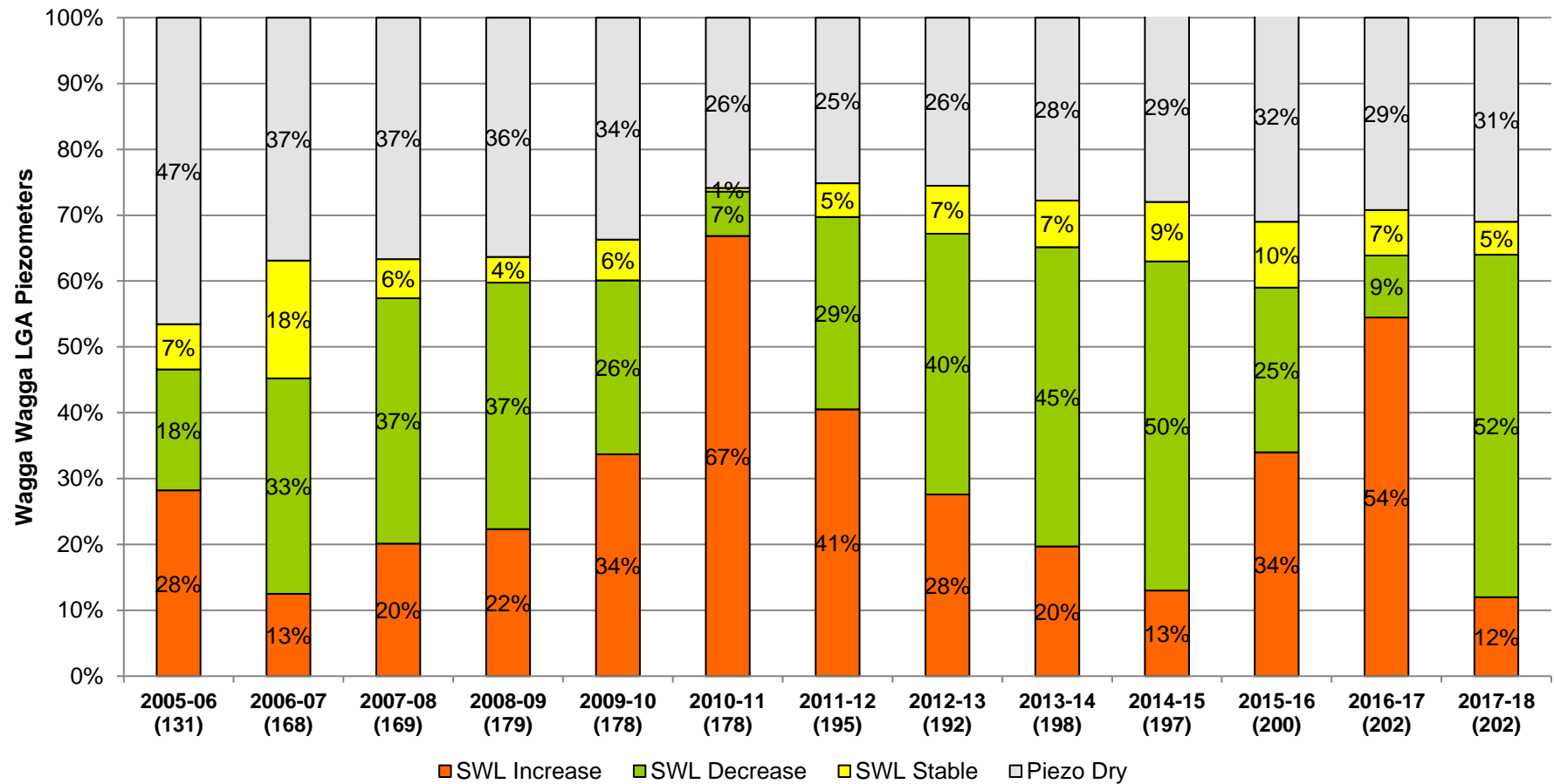
Figure 1: Graph depicting annual change in overall piezometer readings as a percentage of all piezometers in the Wagga Wagga LGA.
