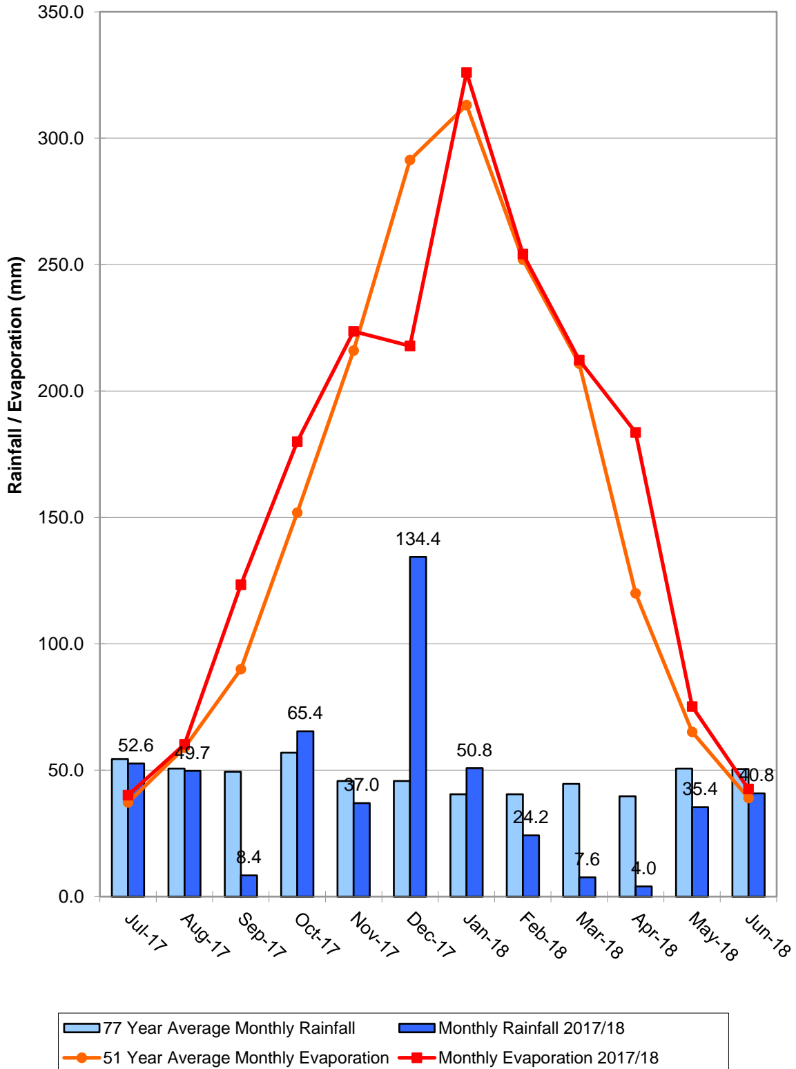
Figure 2: Monthly rainfall and evaporation graph for Wagga Wagga 2017/18.
