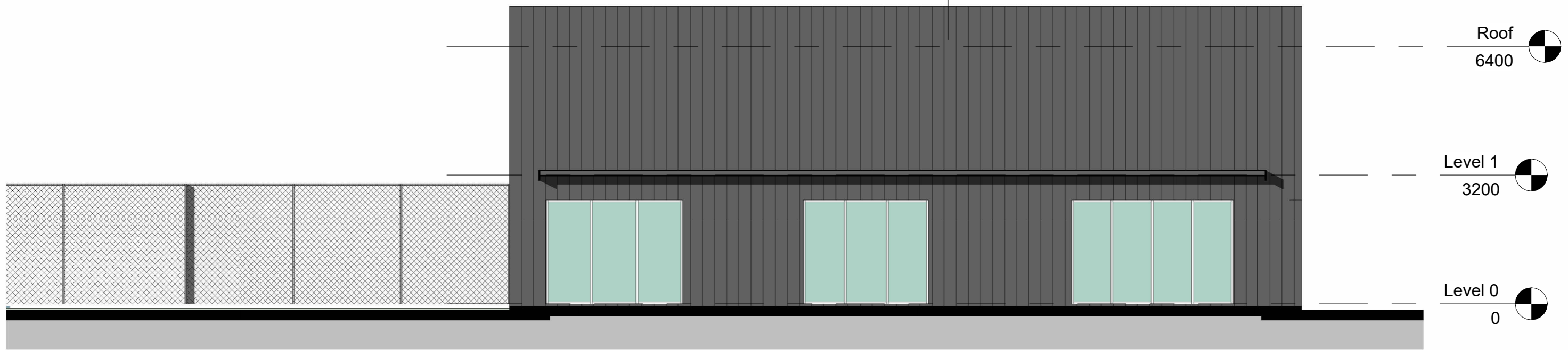
NORTH ELEVATION 1 : 100
