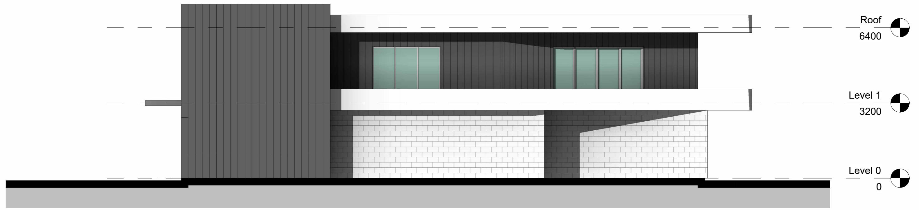
WEST ELEVATION 1 : 100
