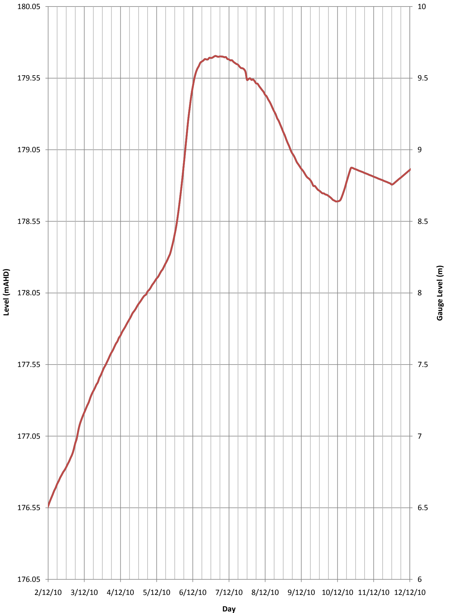
FIGURE 05 HAMPDEN BRIDGE GAUGE
